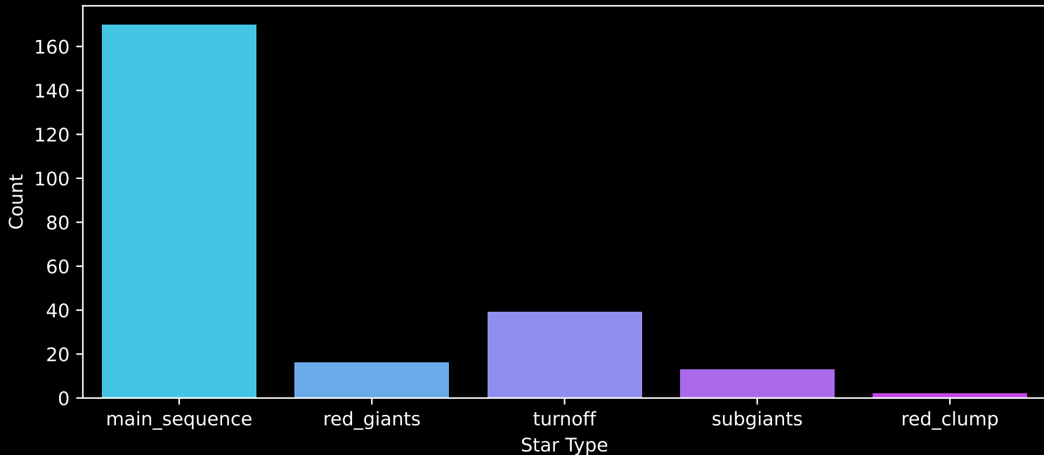
APOGEE DR17 Field: [K2_C12_065-59_btx] Count plot of Star Type
