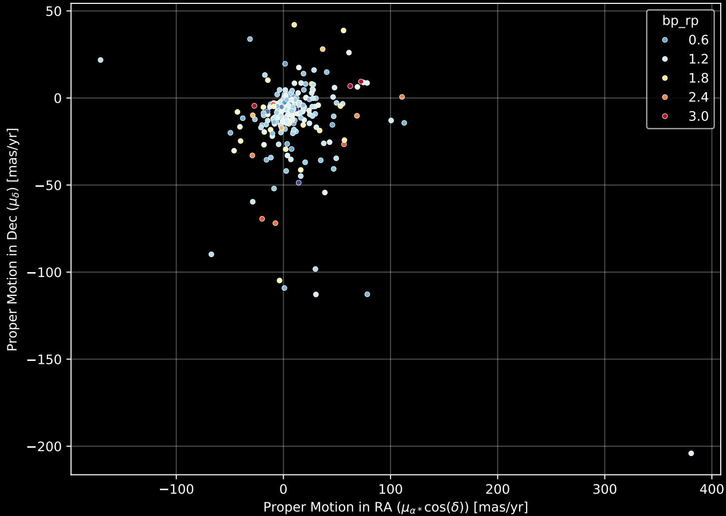
APOGEE DR17 Field: [K2_C12_065-59_btx] Proper Motion Diagram (n= 240)
