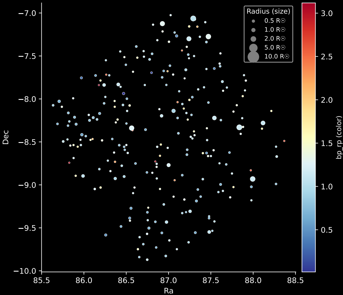
APOGEE DR17 Field: [K2_C12_065-59_btx] Stars: 240
