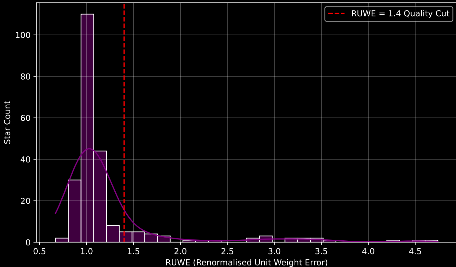
GAPOGEE DR17 Field [K2_C12_065-59_btx] RUWE Distribution (n= 229)
