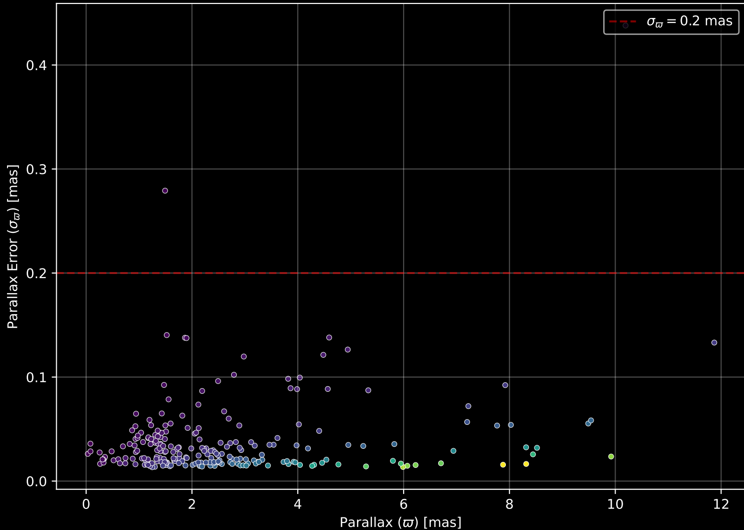
APOGEE DR17 Field: [K2_C12_065-59_btx] Parallax Quality (n= 240)
