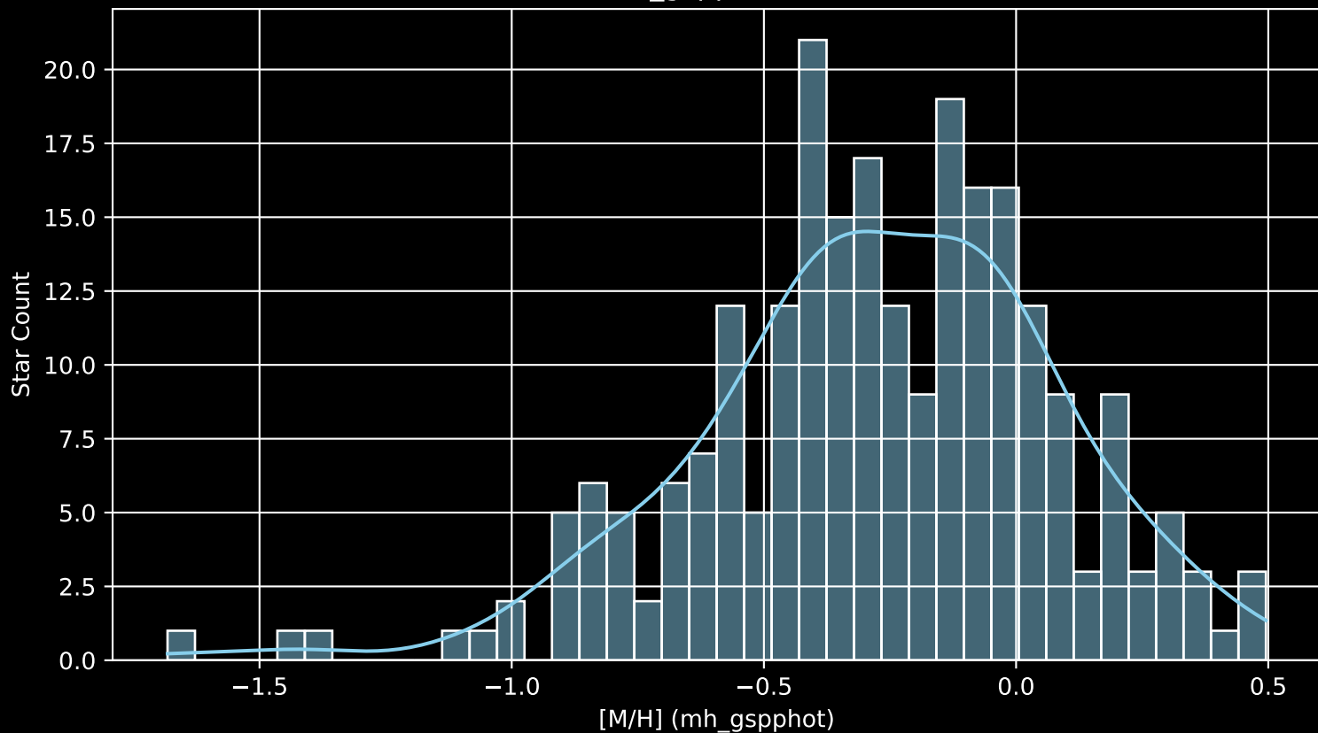
APOGEE DR17 Field: [K2_C12_065-59_btx [M/H] (mh_gspphot) (n= 240)
